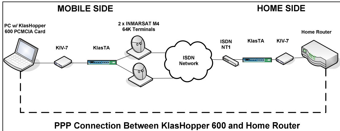
Figure 1. Sample Scenario using the KlasHopper 600 PCMCIA
