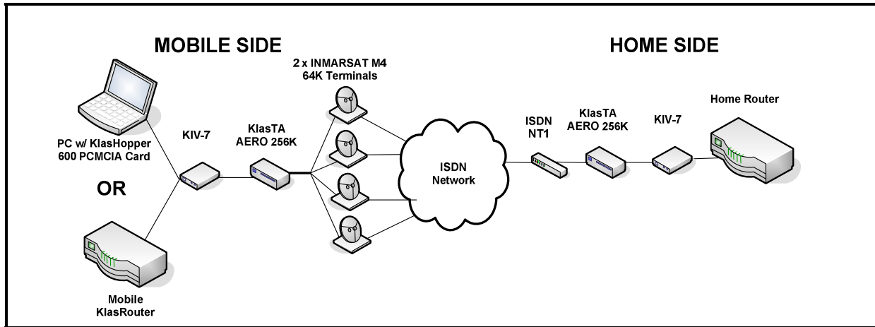
Figure 1. Sample Scenario using the KIV-7 for Type-1 Encryption
